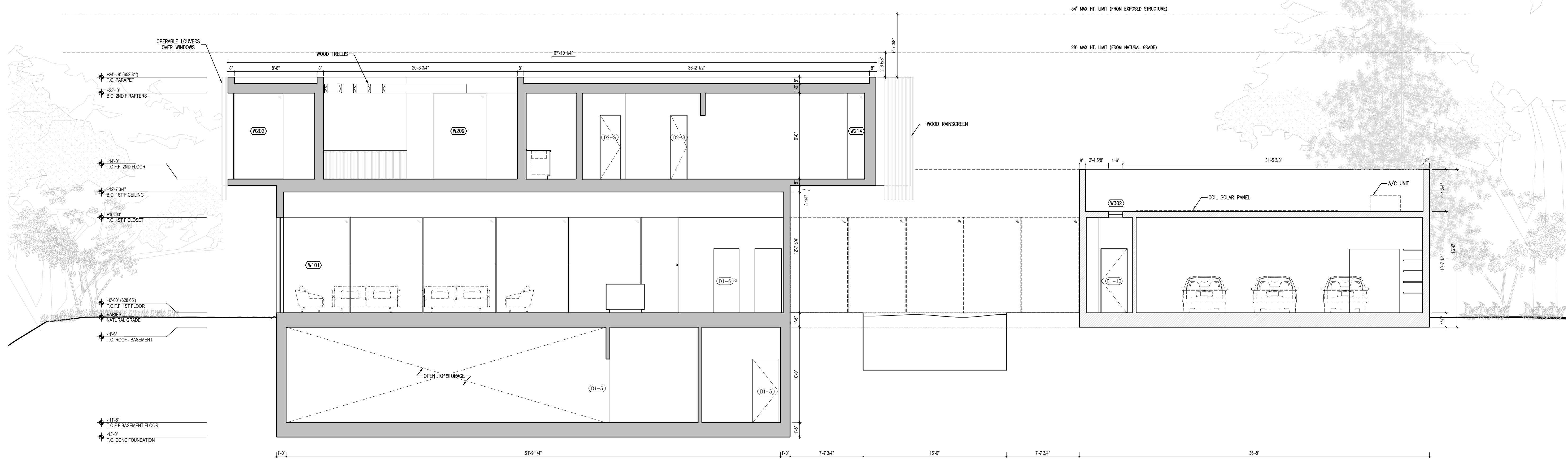
SECTION - LONG PROPOSED
