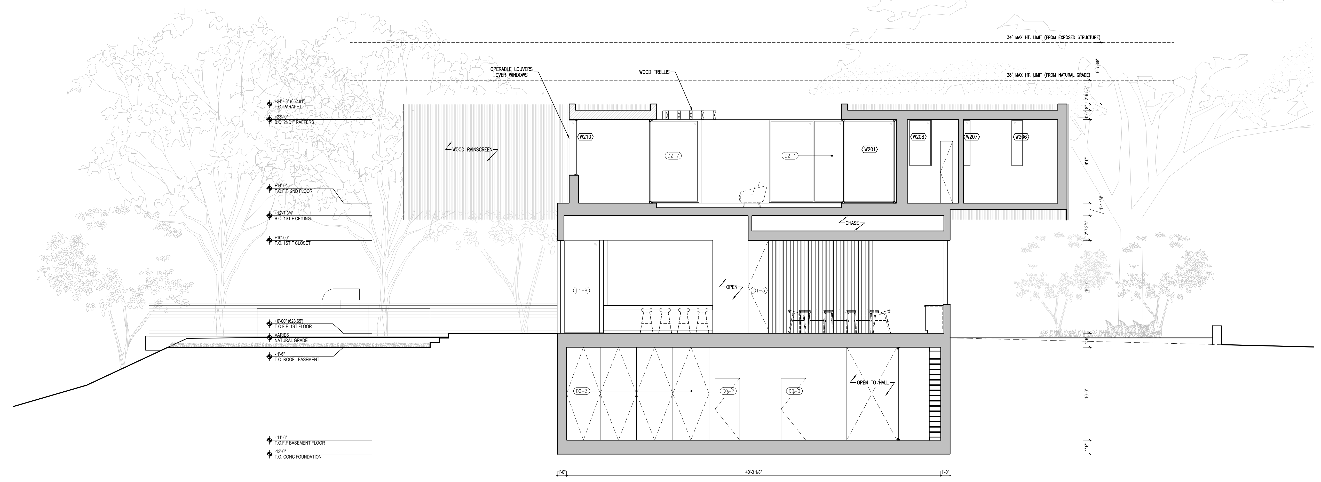
SECTION - SHORT PROPOSED
