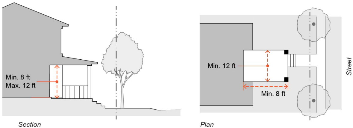
Figure 18.15.060.C.32-b: Porch
