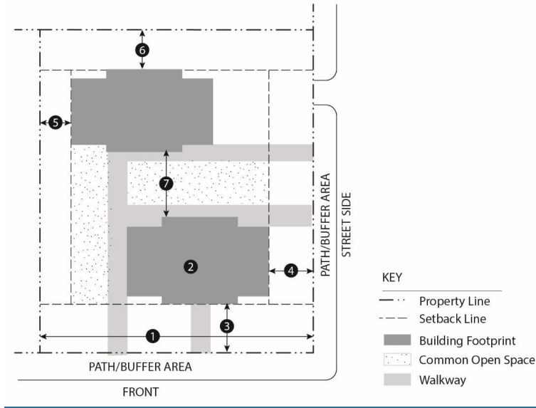
Figure 18.23.050: Development Standards – Mixed-Use Zoning District
