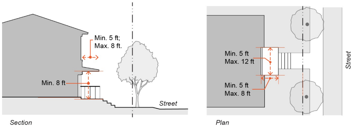
Figure 18.15.060.C.3.c: Stoop
