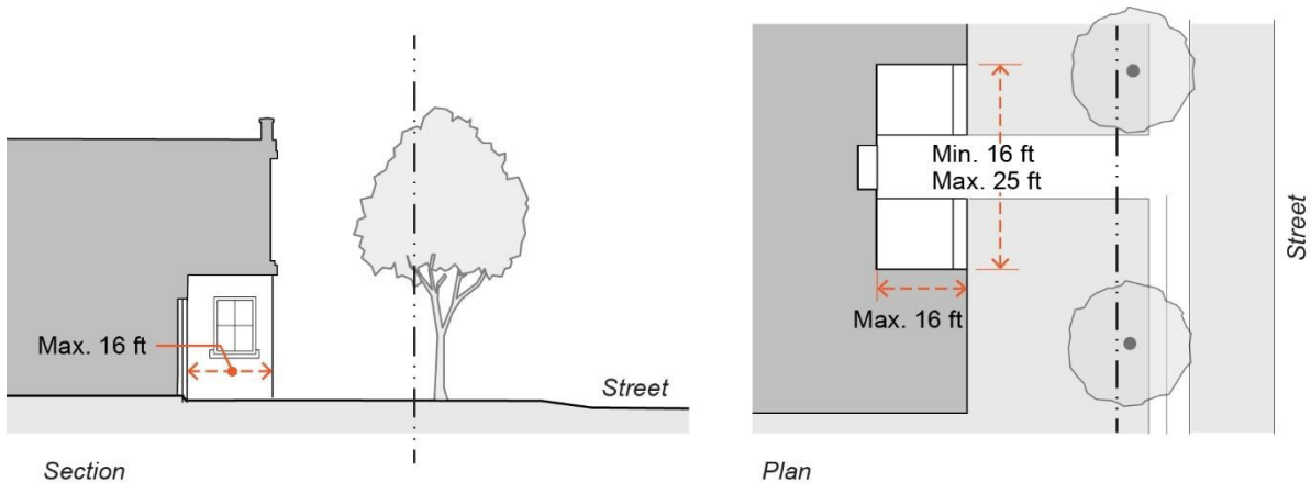
Figure 18.15.060.C.3.d4: Recess
